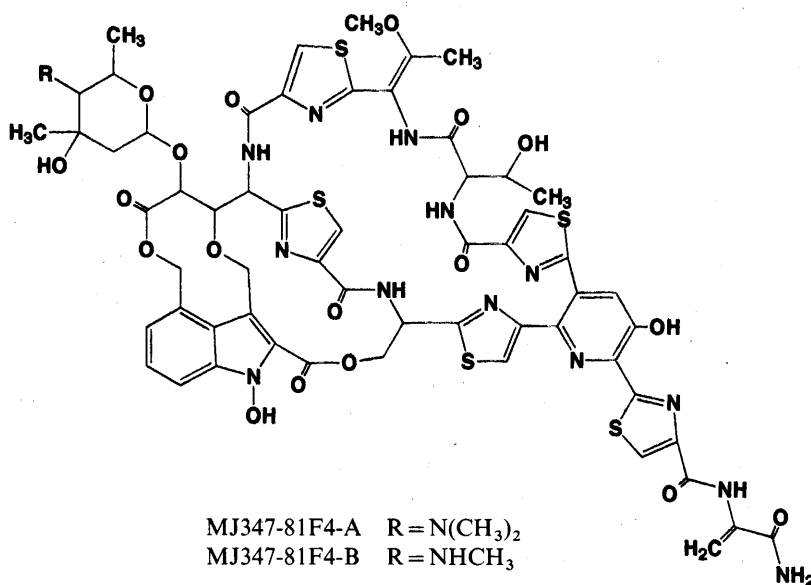
Fig. 1. Structure of MJ347-81F4 components A and B.
